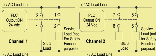
Energized to trip operation D1092D
