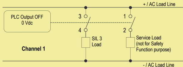
Normal state operation for D1092S
