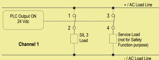
Normal state operation for D1092S
