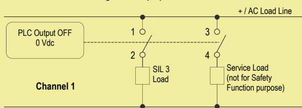
De-energized to trip operation for D1092S
