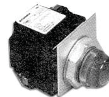
Pilot Light Operator & Lens 100T-PLT1R
